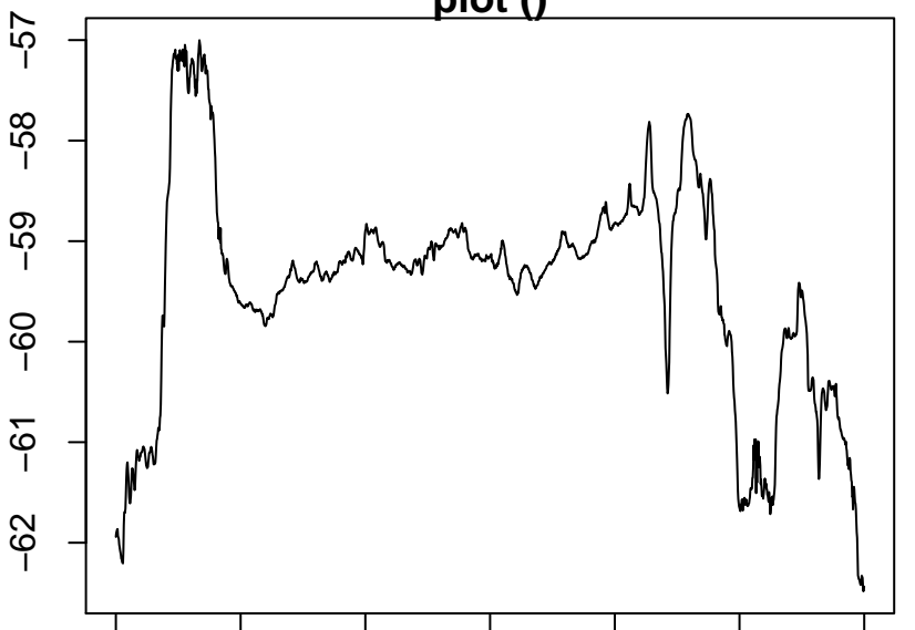
plot ()
